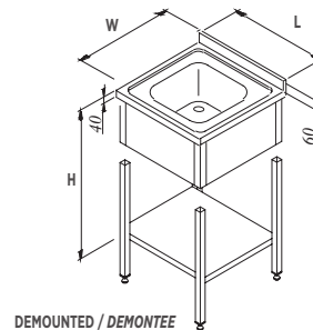
DEMOUNTED / DEMONTEE
