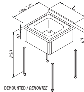
DEMOUNTED / DEMONTEE
