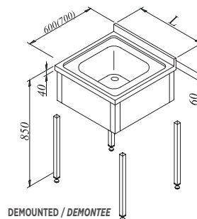
DEMOUNTED / DEMONTEE
