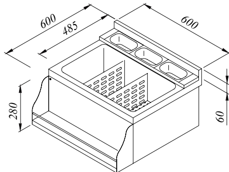
Cocktail Preparation Bench Counter Top Stand de Préparation a Cocktails a Poser
