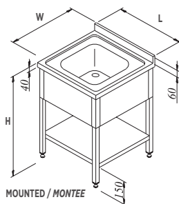
MOUNTED / MONTEE
