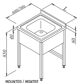
MOUNTED / MONTEE
